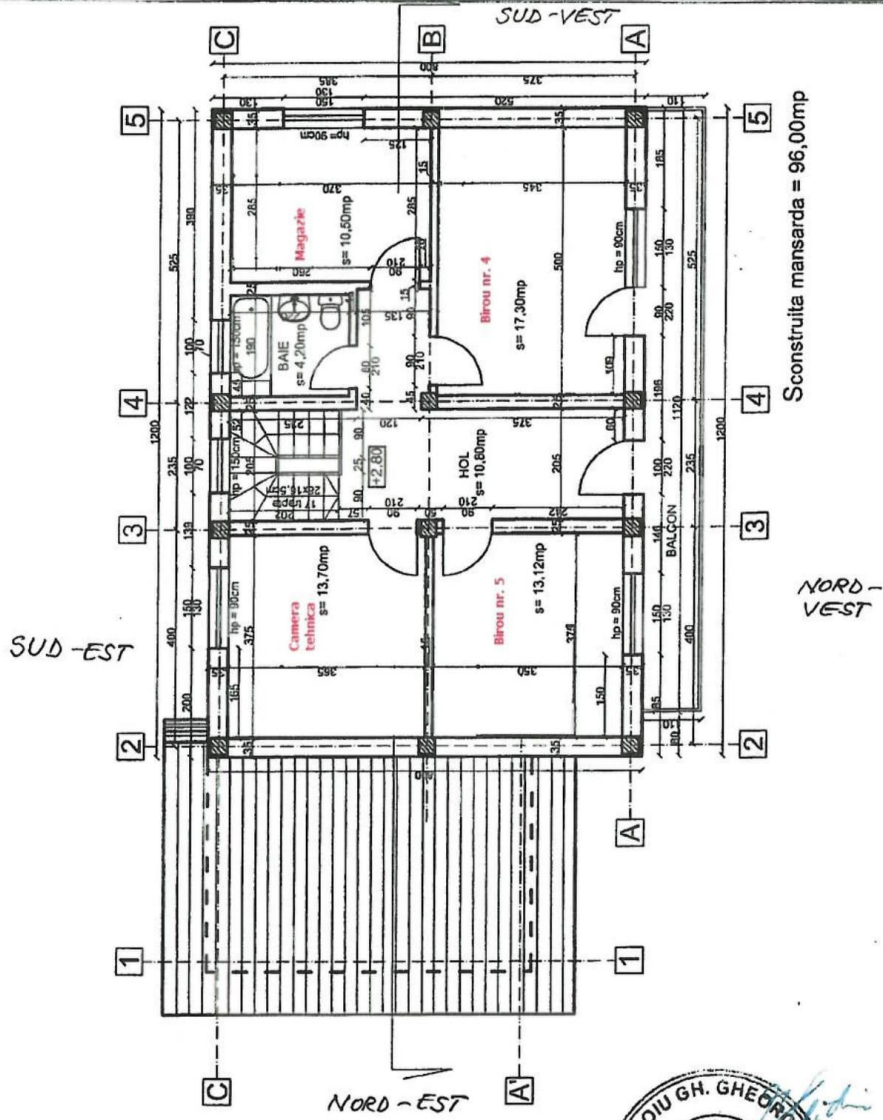
PLAN MANSARDA (Sc 1:100)
