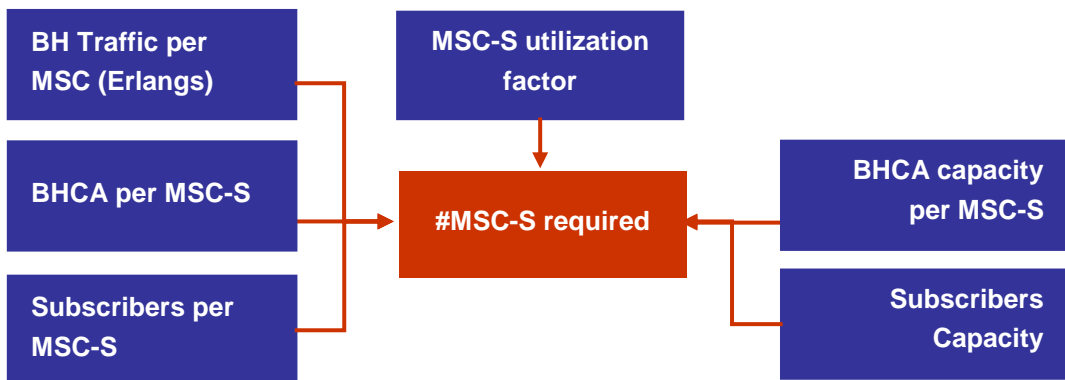
Figure 26 - MSC-S dimensioning
