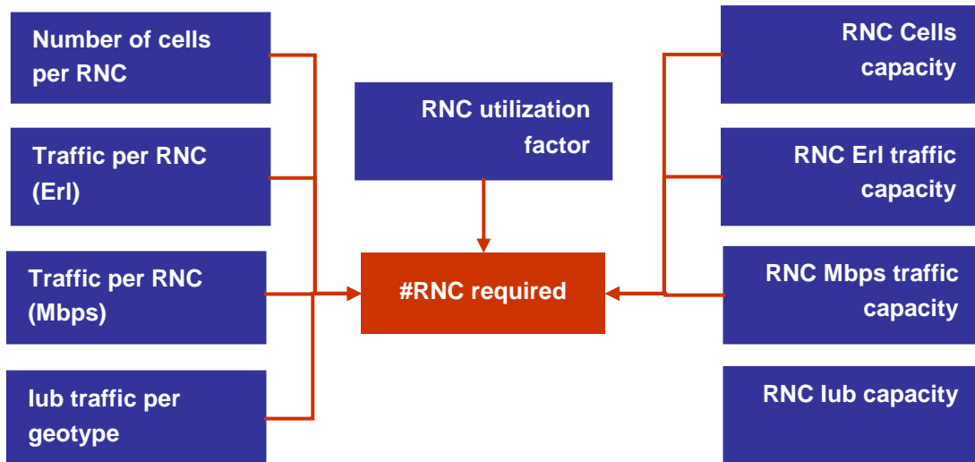
Figure 24 - RNC dimensioning
