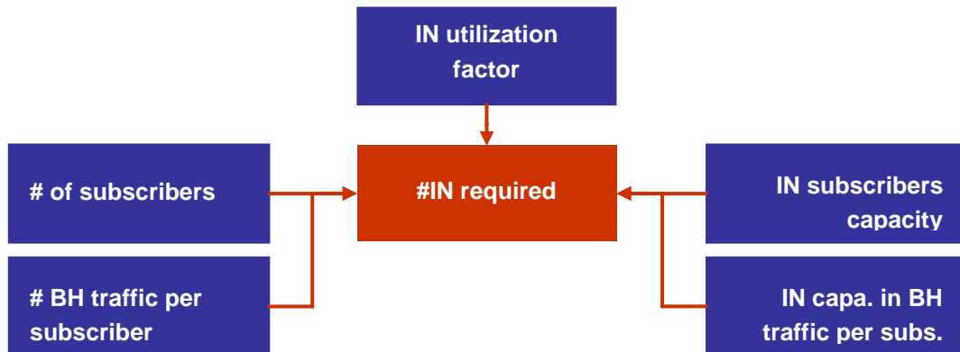
Figure 30 - IN dimensioning
