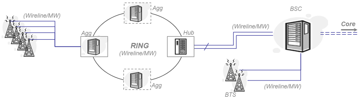
Figure 32 - Access Transmission network physical structure
