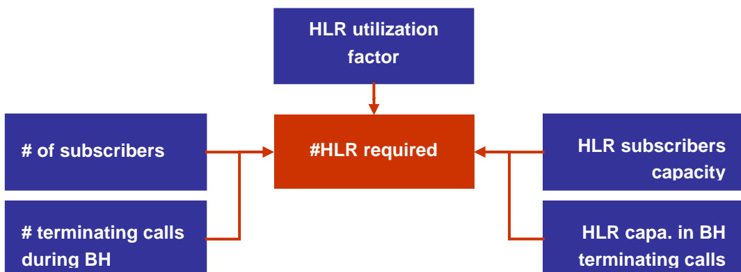
Figure 29 - HLR dimensioning
